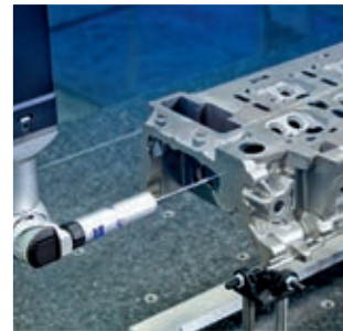
Aluminiumguss- Motorkomponenten Cast aluminium engine components
